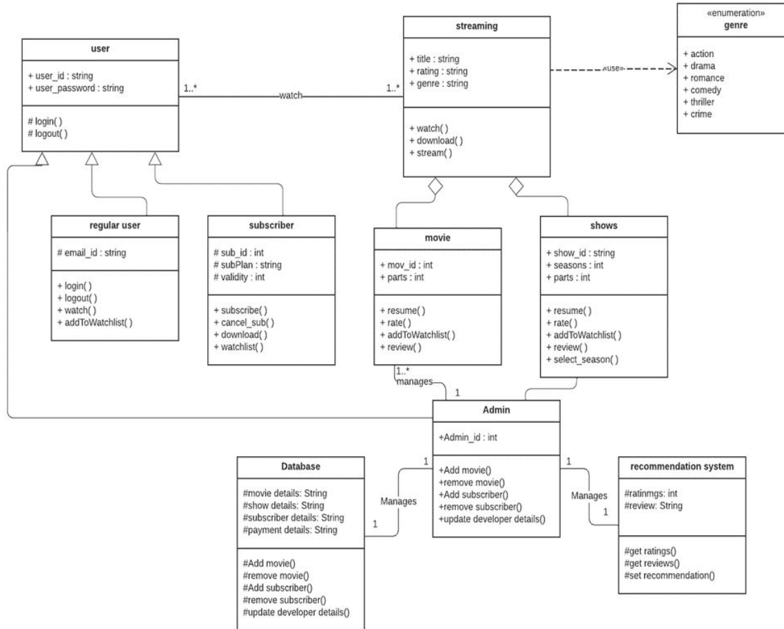
Class Diagram
