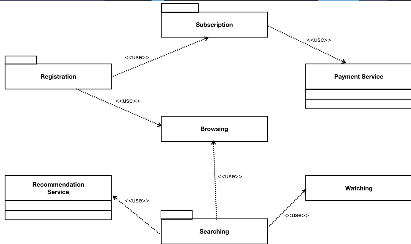
Component diagram
